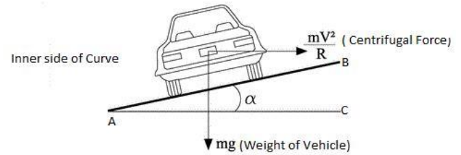
Fig II. Super-elevation on curved portion of road
