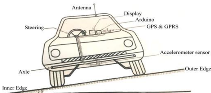
Fig III. Components Parts of Multi-sensory system.
