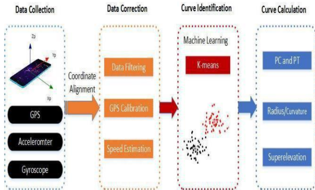
Fig I. System Architecture of C-Finder
