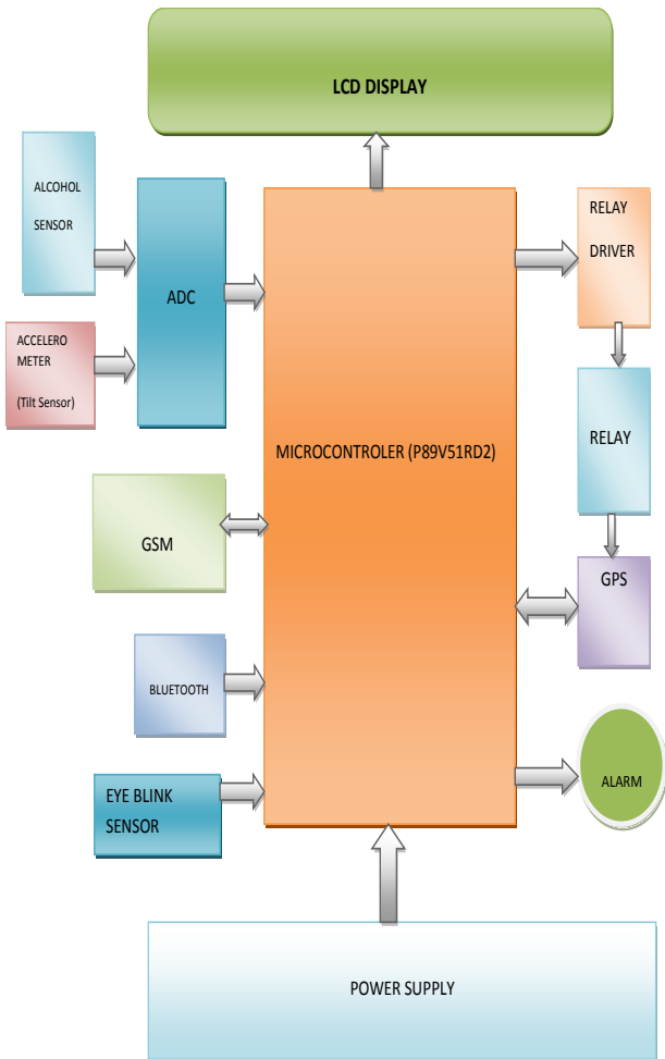
Fig.1. Block Diagram Of Smart Helmet Using GSM, GPS Based System.
